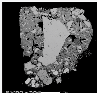
BSE image of entire stratigraphy of BNC_58.
