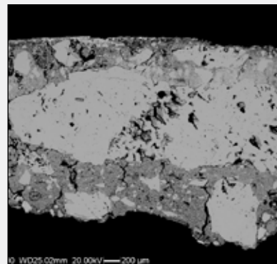
Backscattered electron image of detail of BCN_31R.
