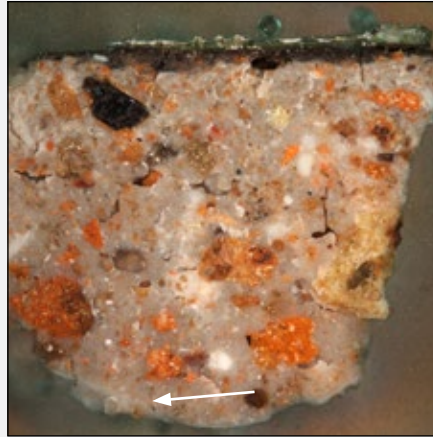
Cross section of BCN_42 (lower south wall, west side) showing the unique plaster found with the brick dust as aggregate. Layer 2 is indicated by the white arrow.
