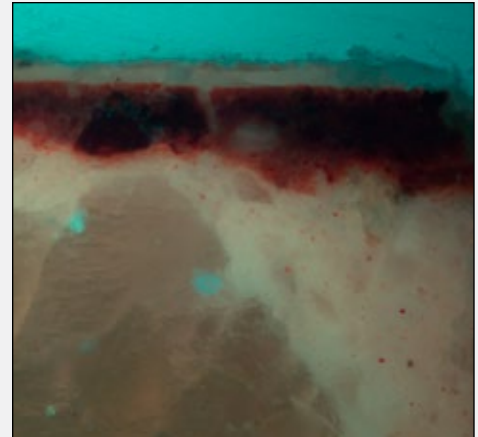
Cross section of BCN_23, seen under UV light, showing the decorative elements applied over a red monochrome background (20x).
