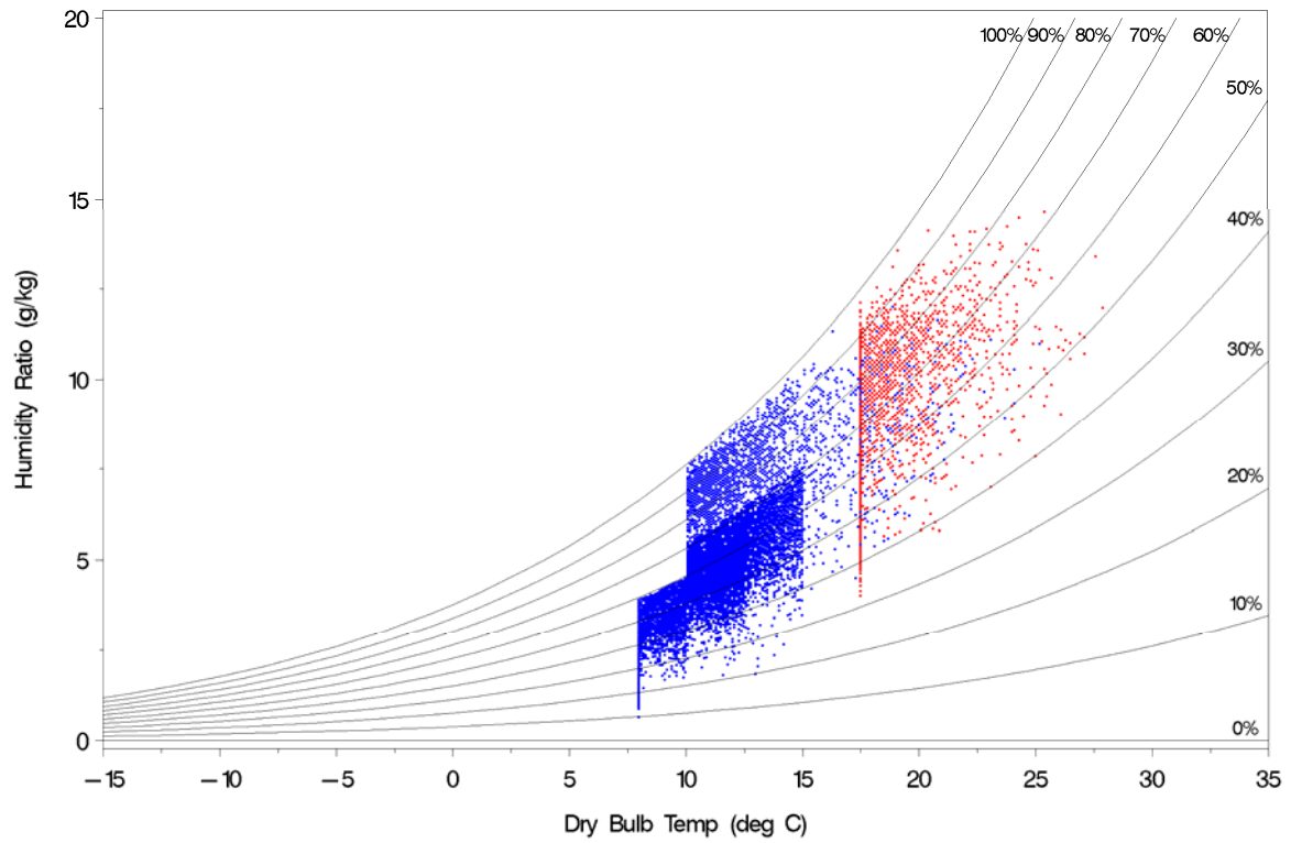
Psychrometric chart showing the modeled indoor climate in Sael and Canal Room with localized heating (January 1901 to December 1952). Data points in blue represent October–May and in red June–September.
